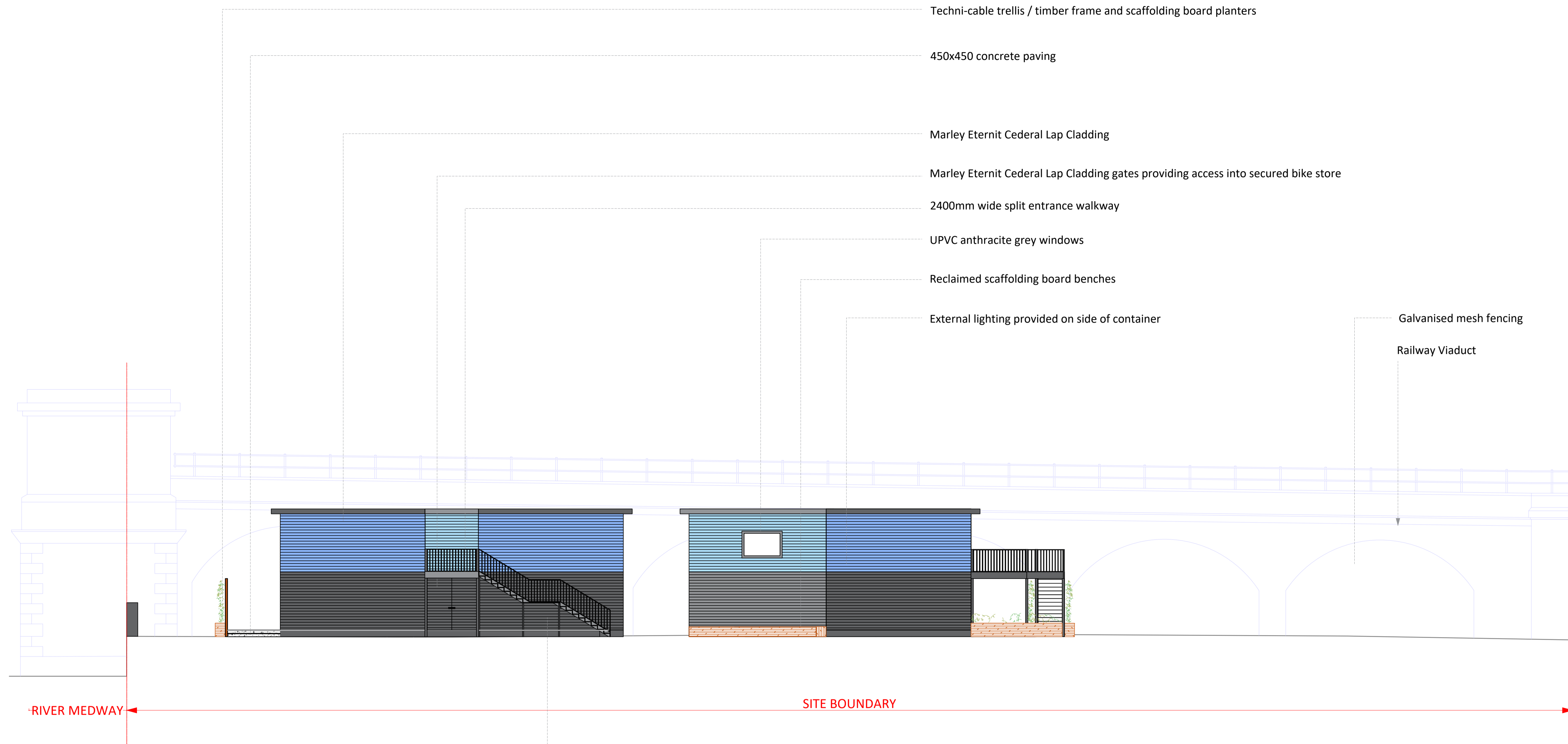
Existing elevation looking Northwest 1:100 @ A1
