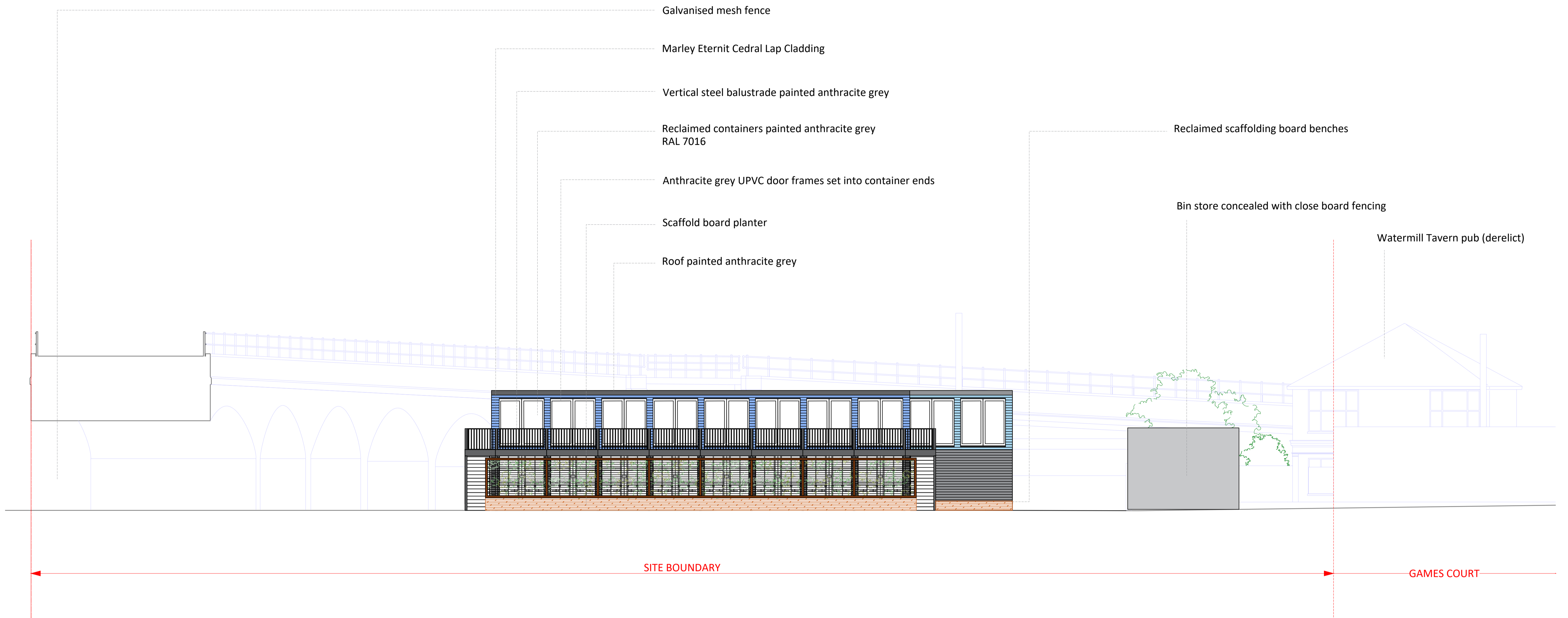
Proposed elevation looking northwest 1:100 @ A1
